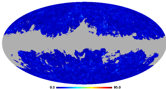
2MASS count map
